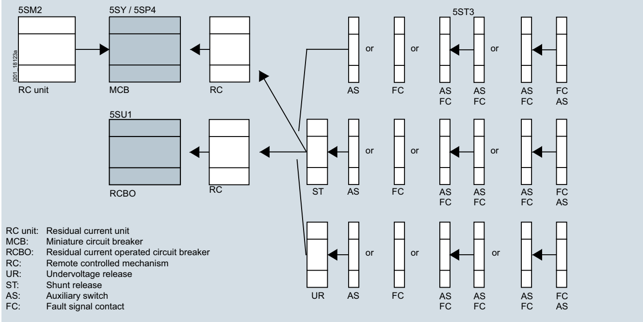
Mounting concept for RCBOs, see chapter "Residual Current Protective Devices / Arc Fault Detection Devices (AFDDs)" in Catalog LV 10.
