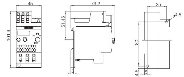
3RU21 26-..C1
