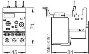
3RB30 26, 3RB31 23, size S0
