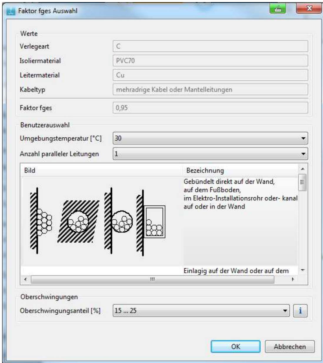
Fig. 2: Screenshot from SIMARIS design showing parameter input for factor f_{tot} (the window is displayed in SIMARIS design by clicking the info button framed in blue in Fig. 1)
