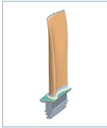
3D-CAD model of Siemens innovative 3D optimized turbine blade stage 3
