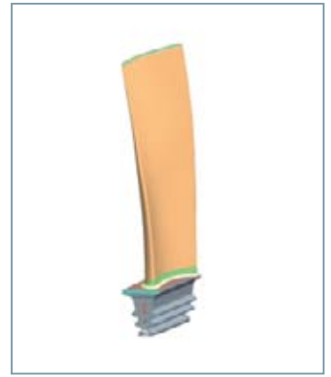
3D-CAD model of Siemens innovative 3D optimized turbine blade stage 4
