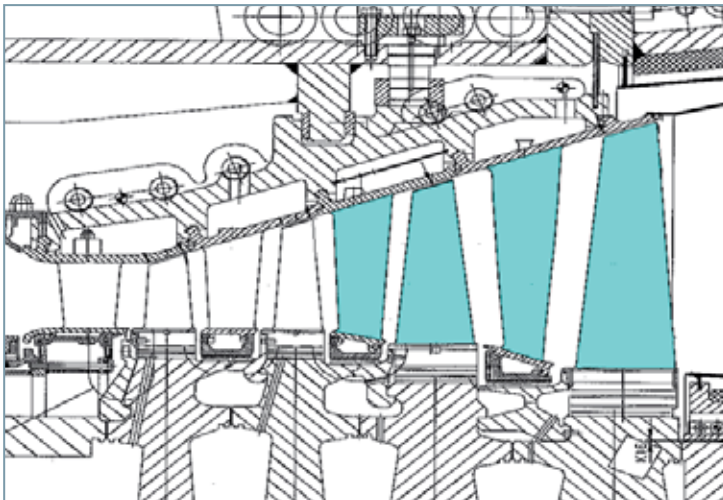
Schematic illustration of Siemens innovative 3D optimized blades and vanes on turbine stages 3 and 4
